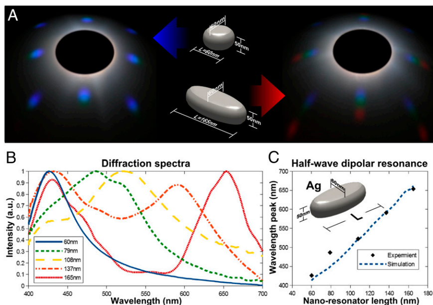
Fig. 1. Spectral characteristics of the scattering of silver nanoparticles. (A) Projected white light diffraction pattern produced by square grids of nanoparticles of 1\text{-}\mu\text{m} pitch. The diffracted light carries the scattering spectrum of the nanoparticle. (B) Measurement of the far-field spectra of nanoparticles of 60 nm in width, 50 nm high, and of multiple lengths. (C) Experimental and simulated plot of the half-wave dipolar resonance peak along the visible spectra.
