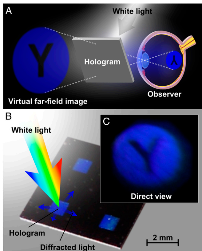
Fig. 2. Narrow-band hologram produced with the scattering of plasmonic nanoparticles when it is illuminated by a white light source. (A) Diagram of the reconstruction of a direct-viewed hologram when it is illuminated with a broad band source. (B) Experimental holograms showing a characteristic blue scattering. (C) Real reconstruction captured with a camera placed in front of the hologram and focused to infinity.
